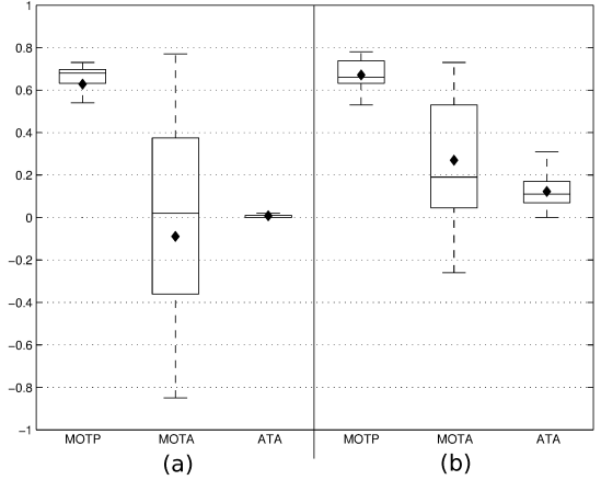
Fig. 1. CLEAR-MOT and ATA metrics for (a) the baseline algorithm and (b) TextSpotter [20], [21], [22] method. Diamond markers indicate average values.
